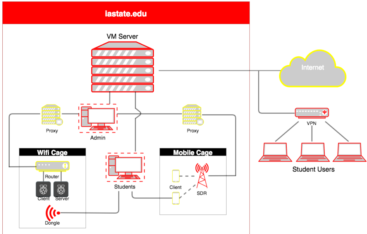
Figure 1: Network Diagram
